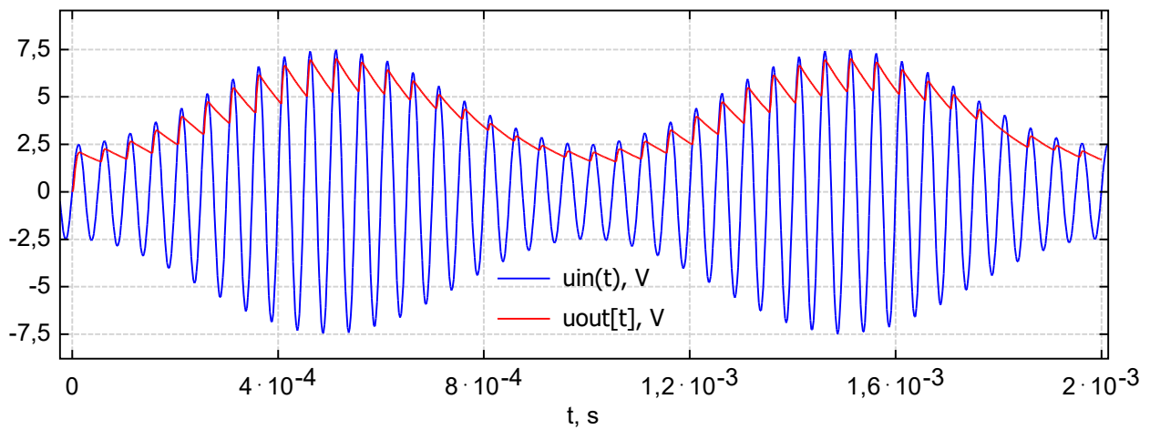
Amplitude detector
